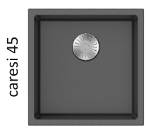
caresi 45 Overall Size : 450mm x 450mm - 17.7" x 17.7" Bowl Size : 400mm x 400mm - 15.7" x 15.7"
